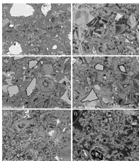
Fig. 1A. Microstructure of PC at 28 days: a) w/b 0.4; b) w/b 0.6; 40% Slag at 28 days; c) w/b 0.4; d) w/b 0.6; 40% Fly ash; e) w/b 0.4; f) w/b 0.6.
