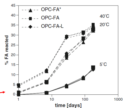
Fig. 3 FA reacted at the different curing temperatures tested
